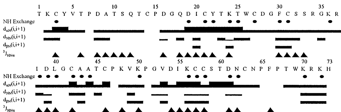
FIG. 2. Amino acid sequence and survey of sequential NOE connectivities in toxin b. Differences in NOE intensities of the sequential d_{\alpha N} , d_{NN} , and d_{\beta N} connectivities are represented by block height . The black circles indicate the amide protons present in the DQF-COSY spectrum, which were recorded immediately after dissolving in D_2O at 10 °C.
